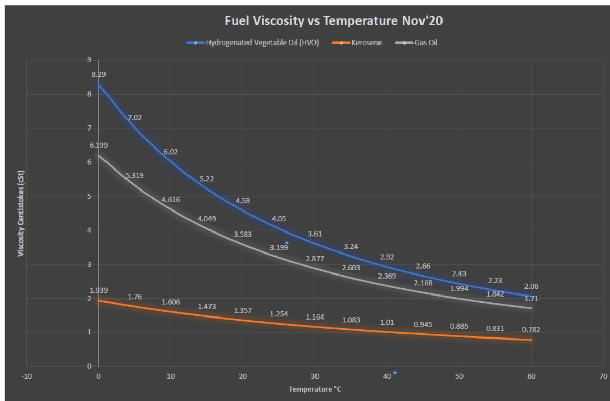
Figure 9: Comparative viscosities of fuels V's temperature
