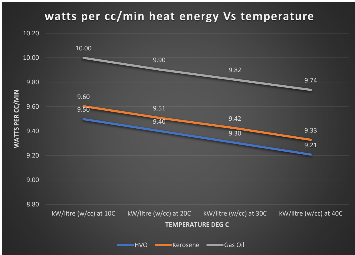
Figure 12: Comparative net heat energy of fuels V's temperature (change in density)
